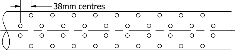
TNZ F2 Drilling pattern (pipe sizes 110mm - 160mm)
