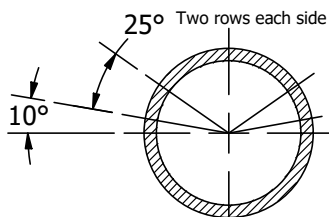
TNZ F2 Drilling pattern (pipe sizes 110mm - 160mm)
