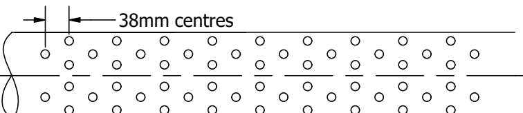
TNZ F2 Drilling pattern (pipe sizes 180mm - 315mm)
