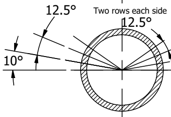
TNZ F2 Drilling pattern (pipe sizes 180mm - 315mm)
